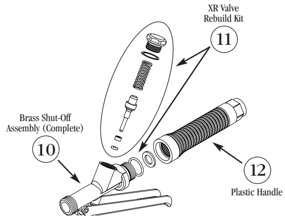
15 Parts Kit
